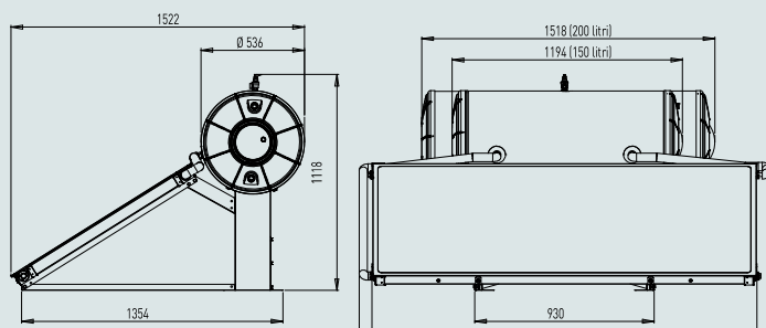
These drawings refer to 150/1 and 200/1 models
